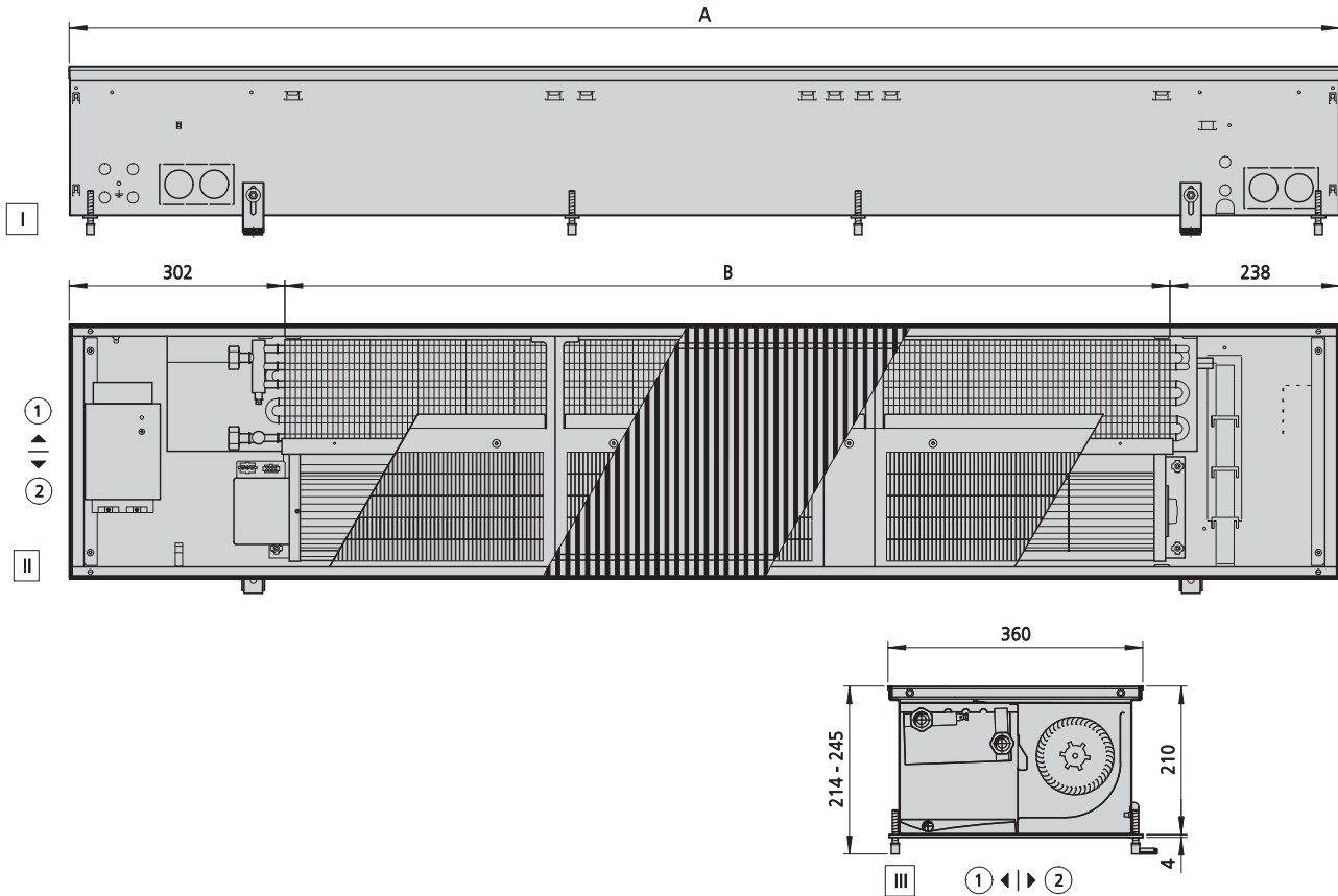
Technical drawing (Dimensions in mm)
