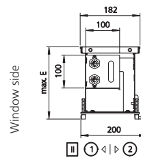
Cross-section through trench height 150/200 mm (example shown with roll-up grille)
