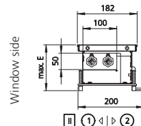
Cross-section through trench height 92/120 mm (example shown with roll-up grille)
