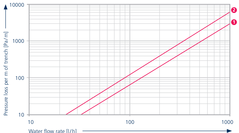
1 Trench height 92 mm/120 mm 2 Trench height 150 mm/200 mm
