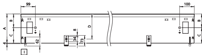
Front view of trench height 150/200 mm
